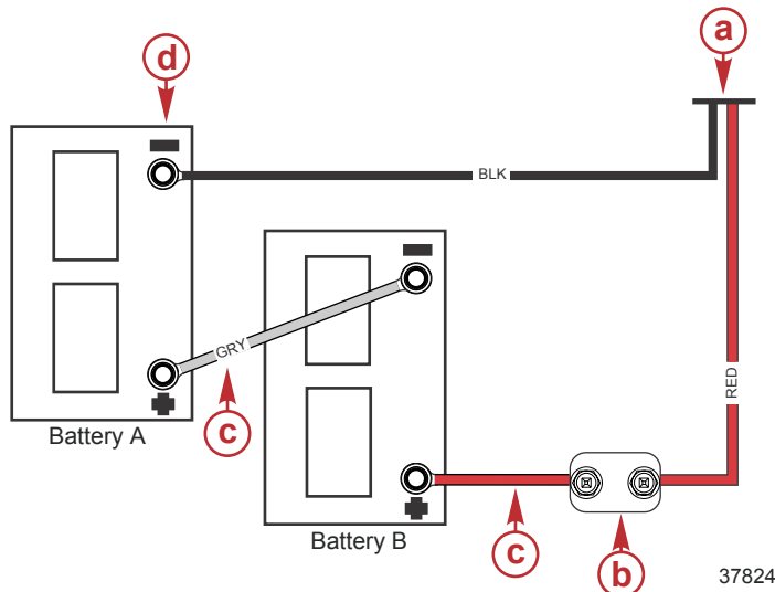
24-volt battery connection
