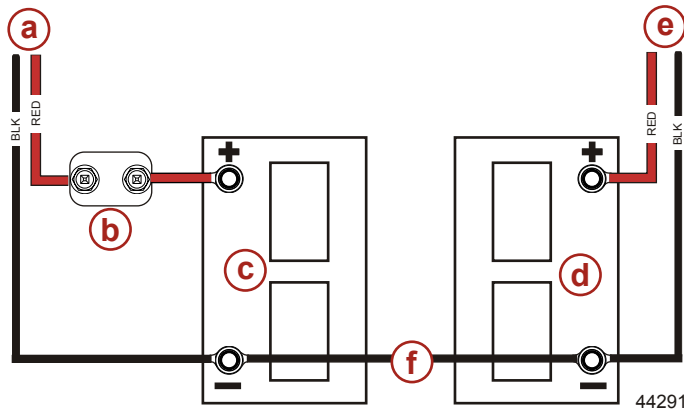
12-volt battery connection with common ground bond
